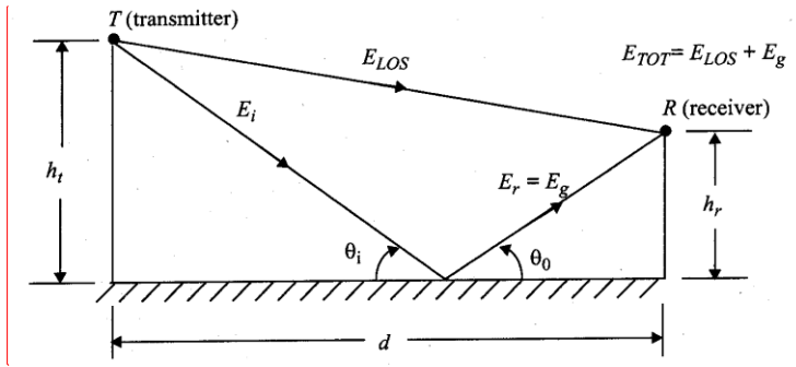
Figure 1.1: Two Ray Model
